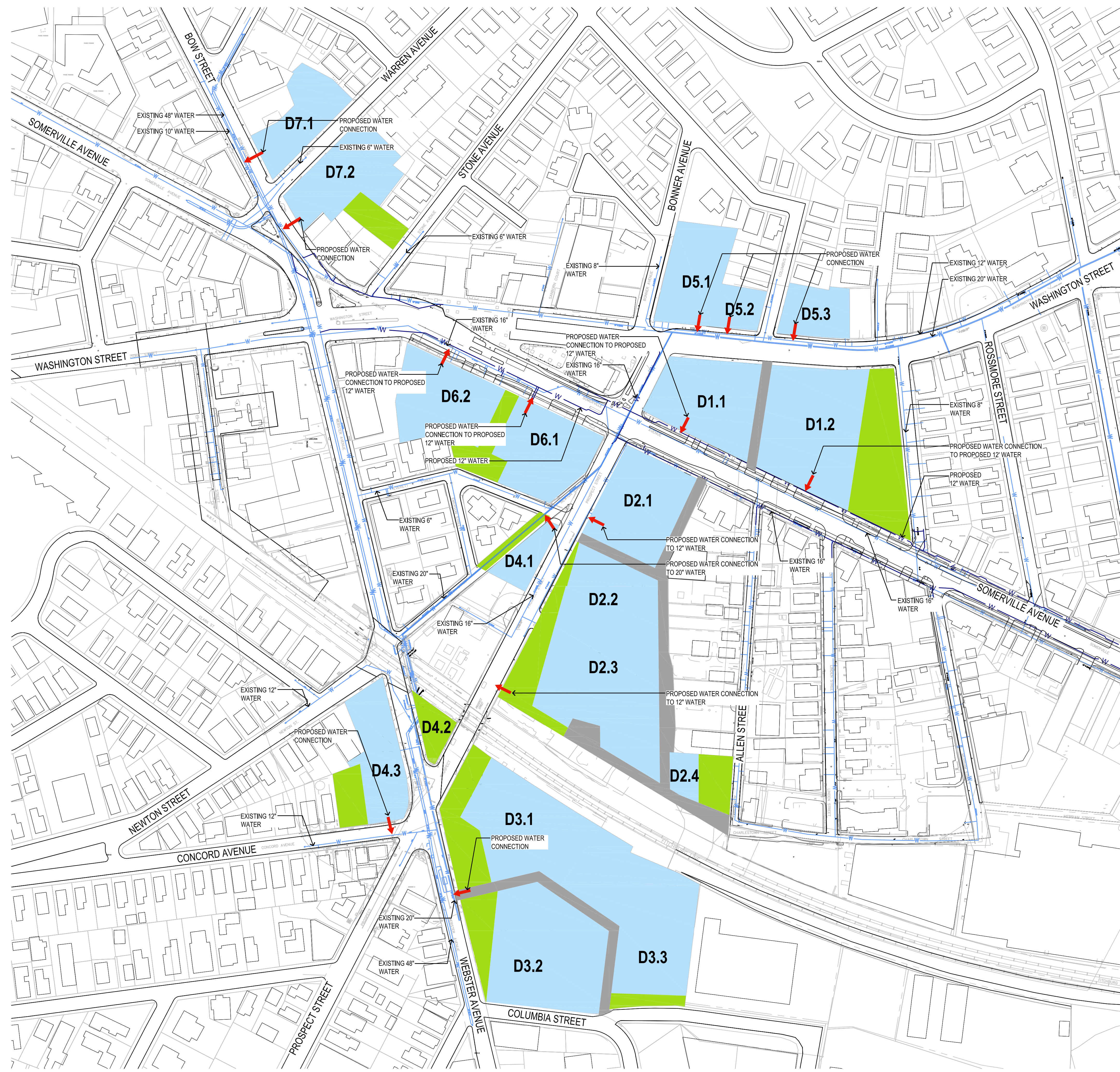
OVERALL WATER SYSTEM PLAN 1" = 100'-0"
