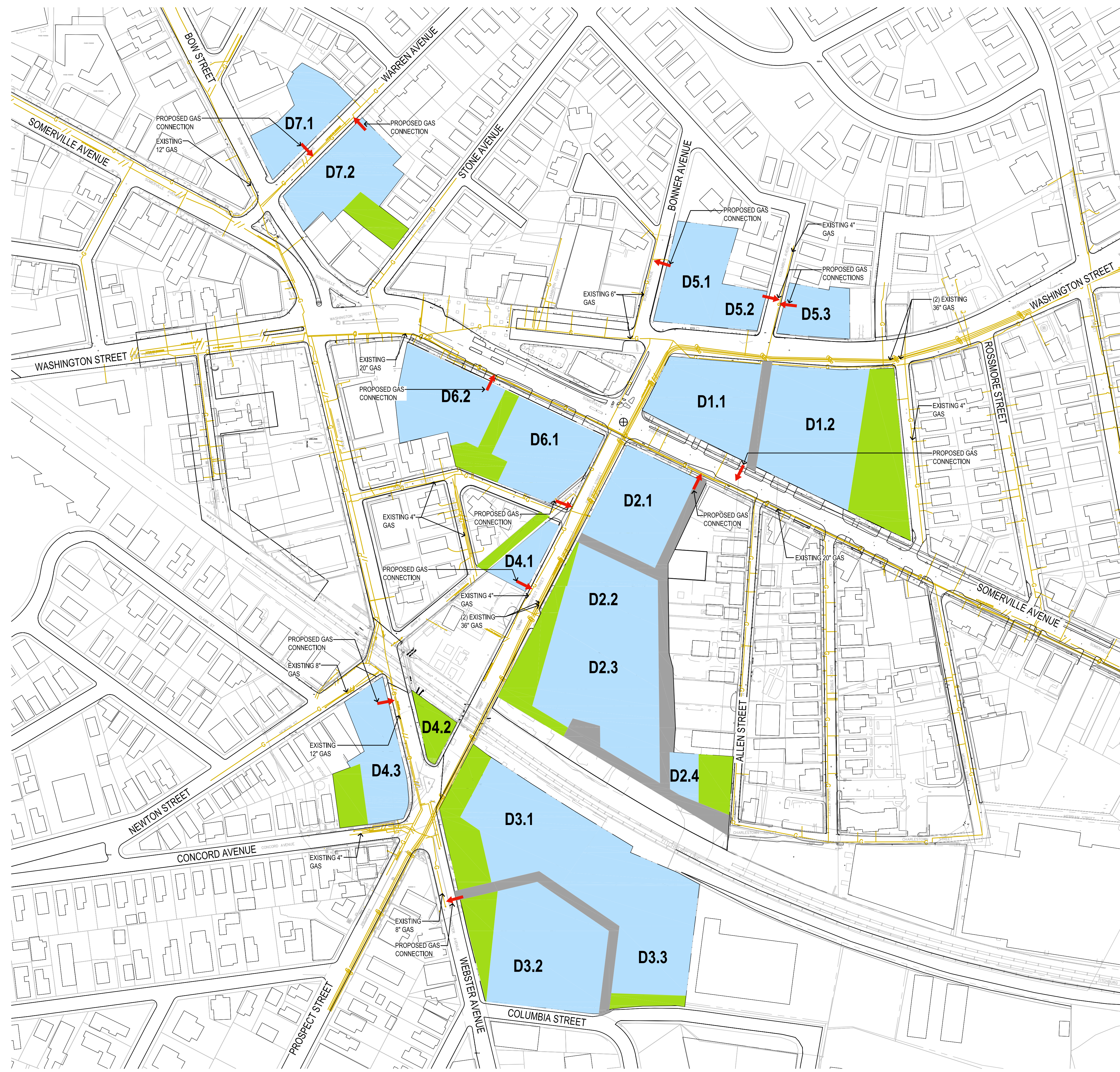
OVERALL GAS PLAN 1" = 100'-0"
